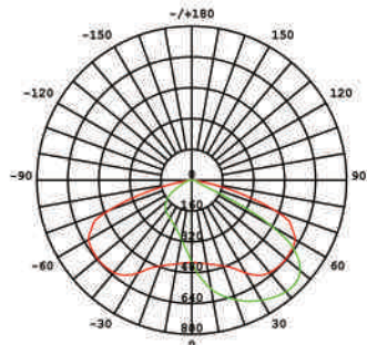
AVERAGE BEAM ANGLE(50%):108.3DGE UNIT: cd — C0/180, 151.7° I 0 :426.3 — C90/270, 84.9° I 0 :759.2
